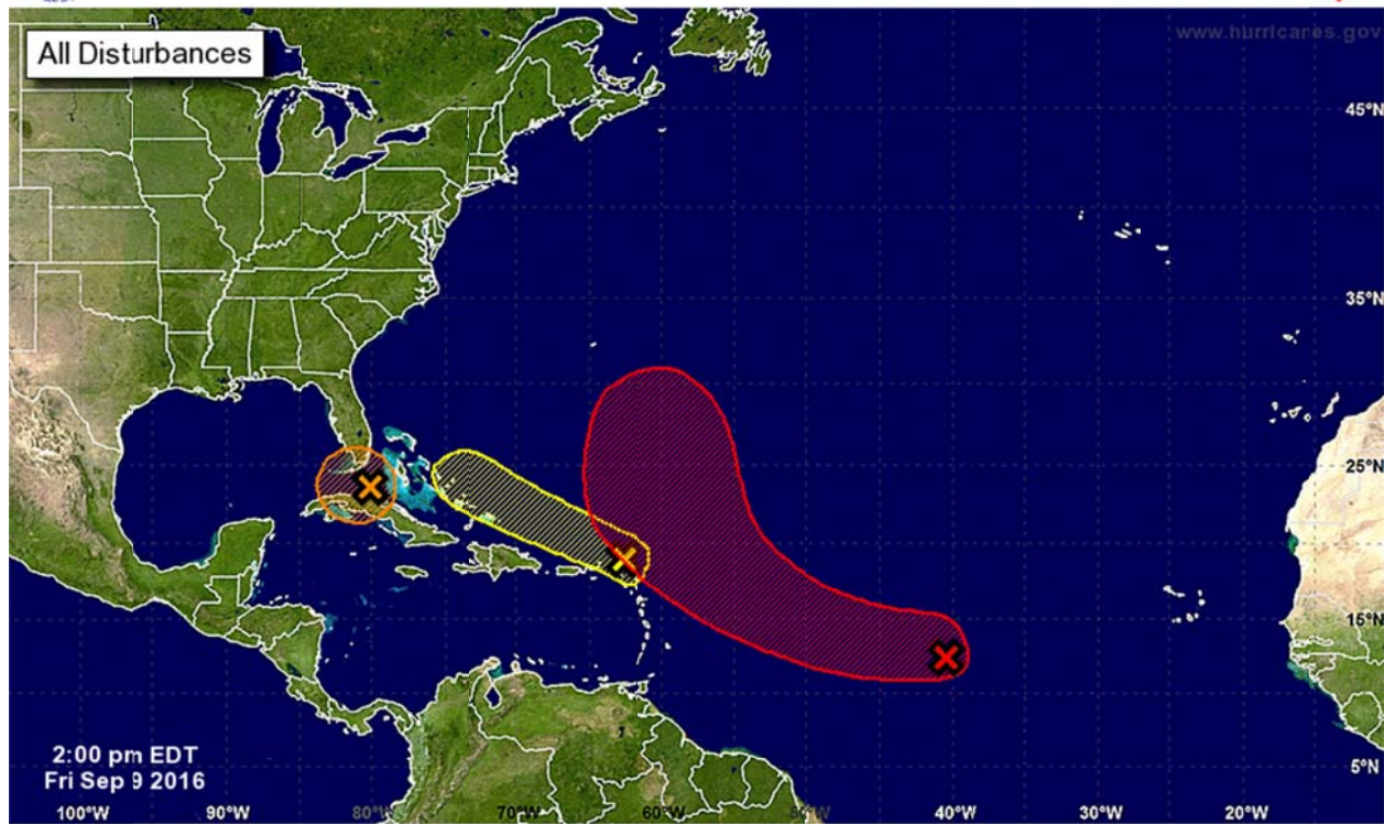
Tropical Cyclone Formation Potential for the Five-Day Period Ending at 2:00 pm EDT Wed Sep 14 2016 Chance of Cyclone Formation in Five Days: ■ Low < 40% ■ Medium 40-60% ■ High > 60% X indicates current disturbance location; shading indicates potential formation area.
